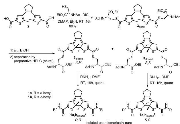
Scheme 2. Synthesis of the sergeants 1a closed § and 1b closed § . DIC = N,N' -diisopropylcarbodiimide, DMAP = 4-( N,N -dimethylamino)pyridine.
