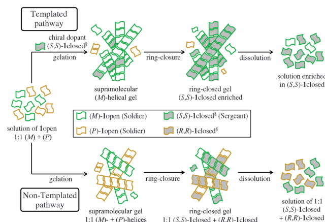
Figure 1. Concept for autoamplification of molecular chirality through the induction of supramolecular chirality. For the templated pathway, a small fraction of chiral dopant ( S,S )- 1 closed § is added to a mixture of prochiral photoswitches [( M )- 1 open and ( P )- 1 open ] prior to gelation. The formed fibers that result in gel formation are templated by the chiral dopant ( S,S )- 1 closed § and one helicity ( M ) is dominant. Upon ring closing of the photoswitches with UV light, the chirality of the fibers results predominantly in the formation of the templated enantiomer ( S,S )- 1 closed § . If no chiral dopant is added to the mixture of prochiral photoswitches (non-templated pathway), the gel is made up of an equal mixture of P and M conformers in the fibers. Subsequent ring closure results in a statistical 1:1 mixture of products.
